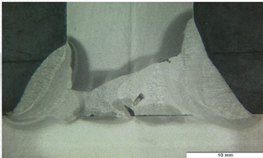
Defects: lack of sidewall and inter run fusion and lack of root penetration
