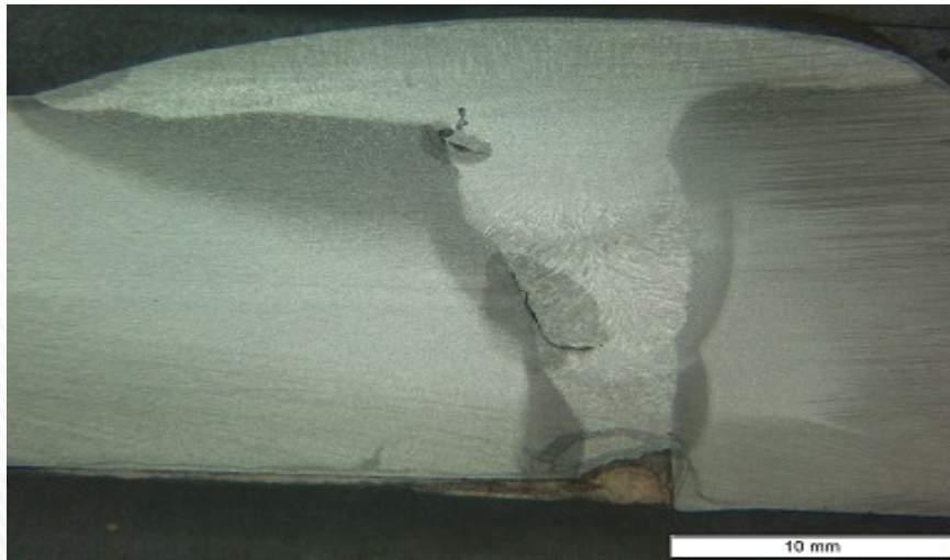
Defects: lack of sidewall and inter run fusion and lack of root penetration
